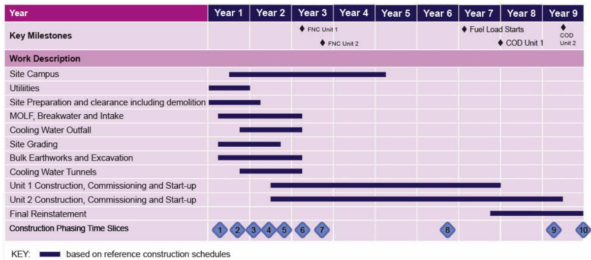
Figure 2-1 Indicative construction timeline for the Wylfa Newydd Development Area
