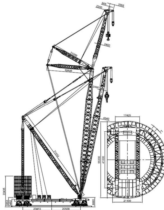
Figure 3-3 Typical section and plan view of very heavy lift crane
